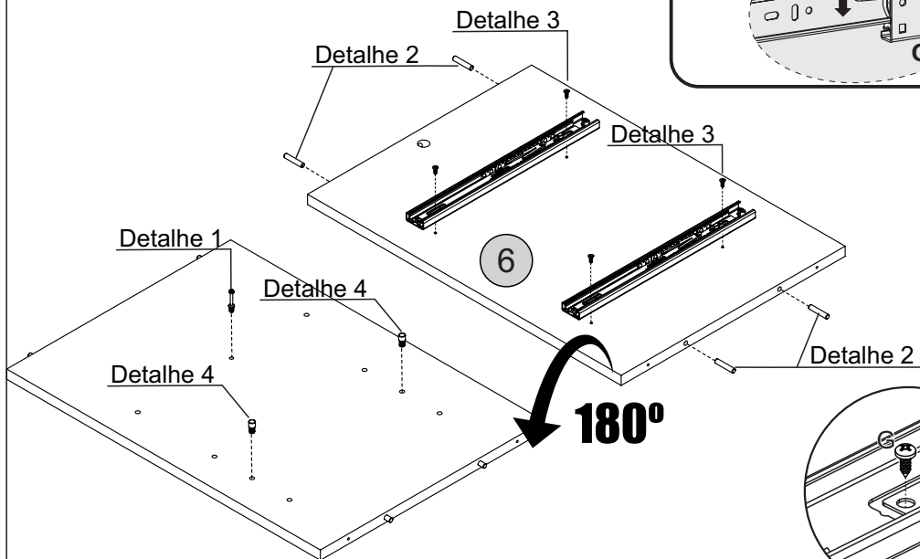
Detalhe 3 Detalle/Detail
