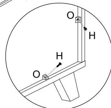
Detalhe 17 Detalle/Detail
