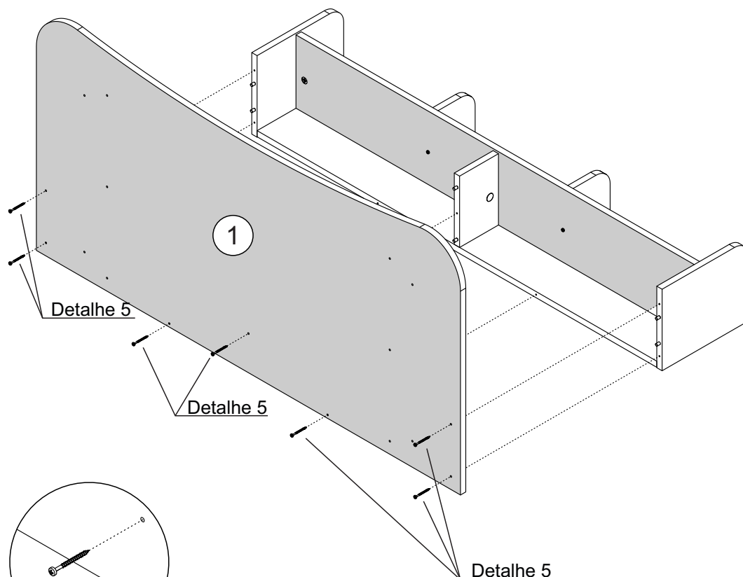
Detalhe 5 Detalle/Detail
