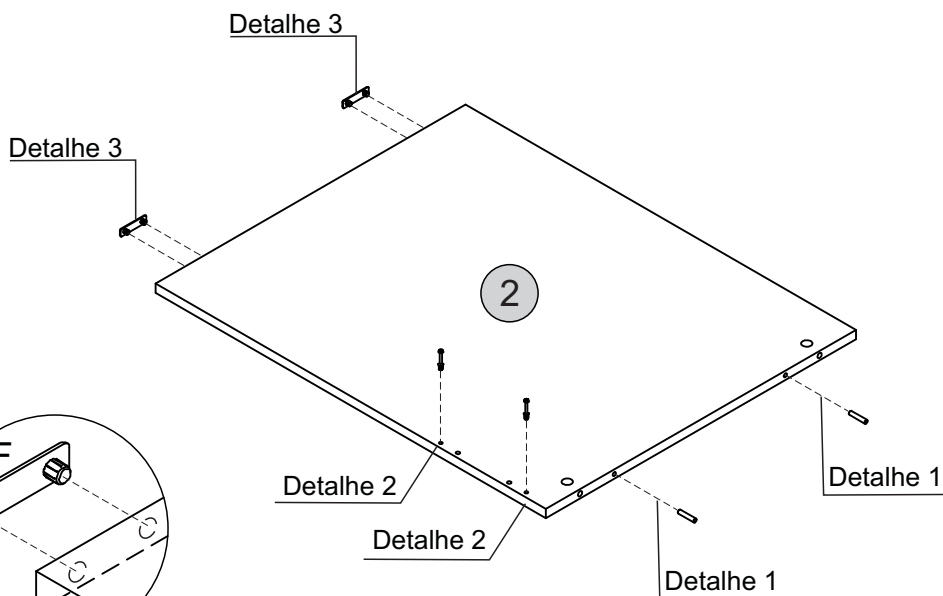
Detalhe 3 Detalle/Detail
