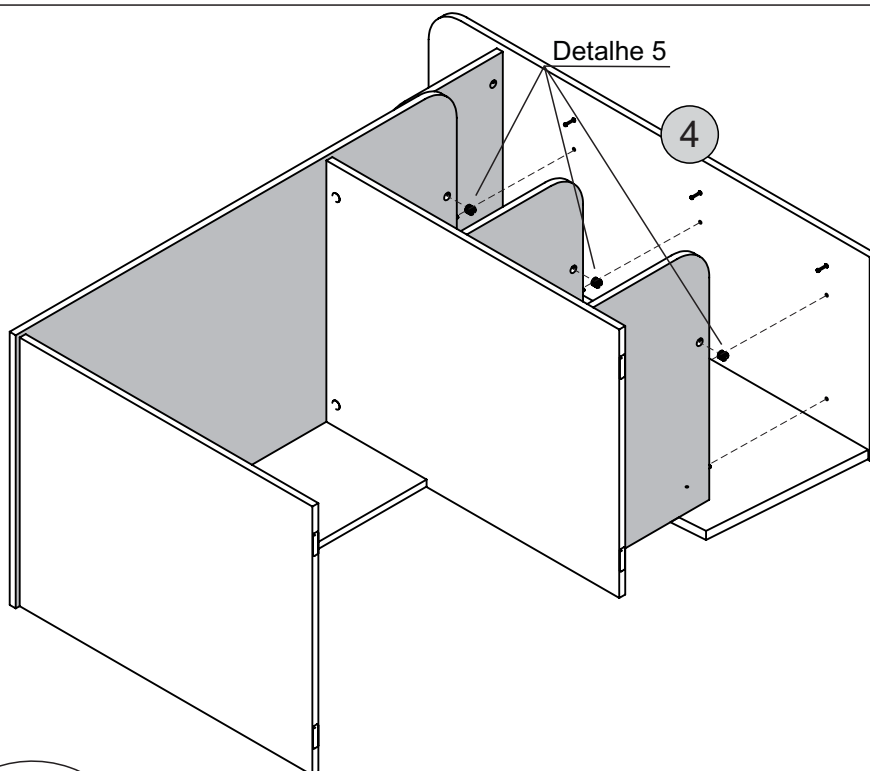
Detalhe 5 Detalle/Detail
