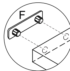
Detalhe 3 Detalle/Detail
