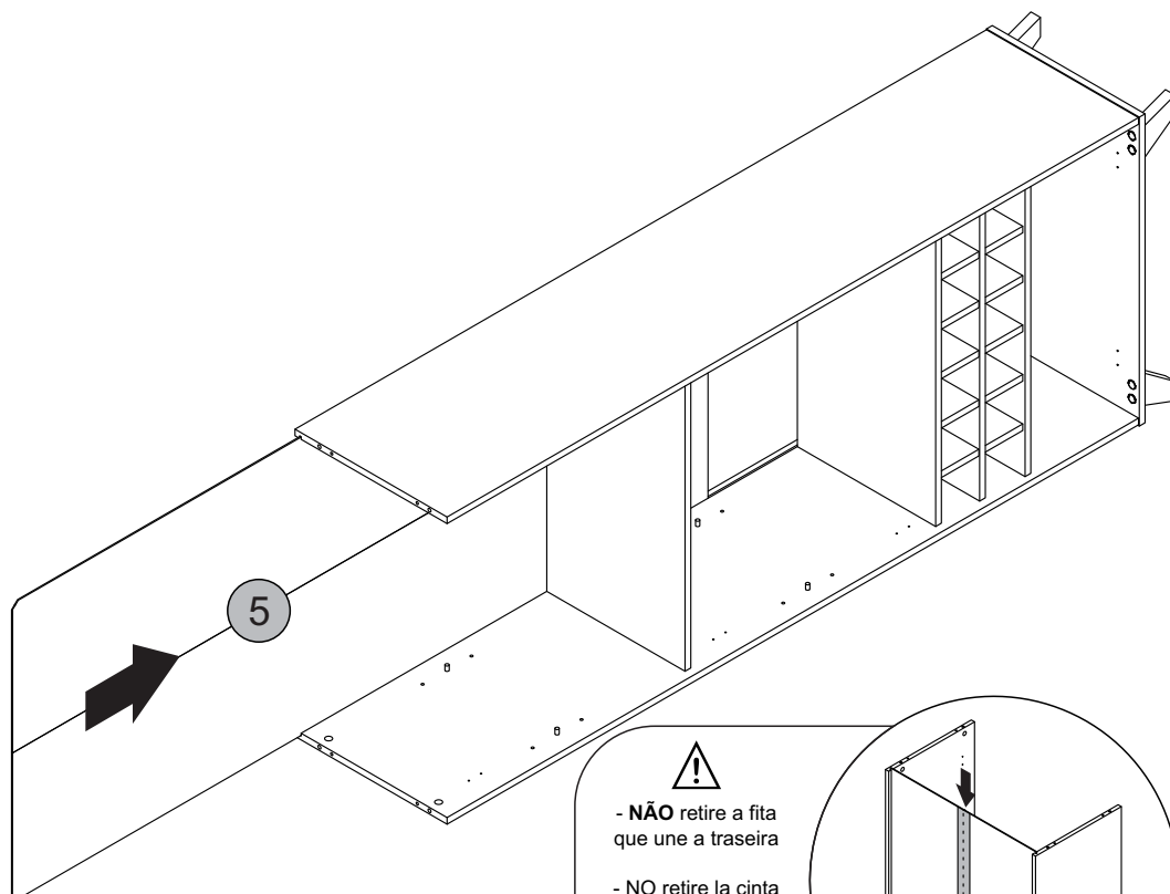
Detalhe 11 Detalle/Detail
