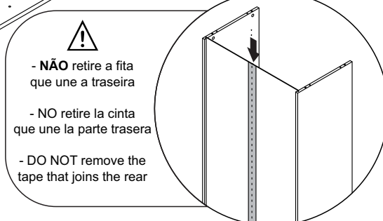
Detalhe 11 Detalle/Detail
