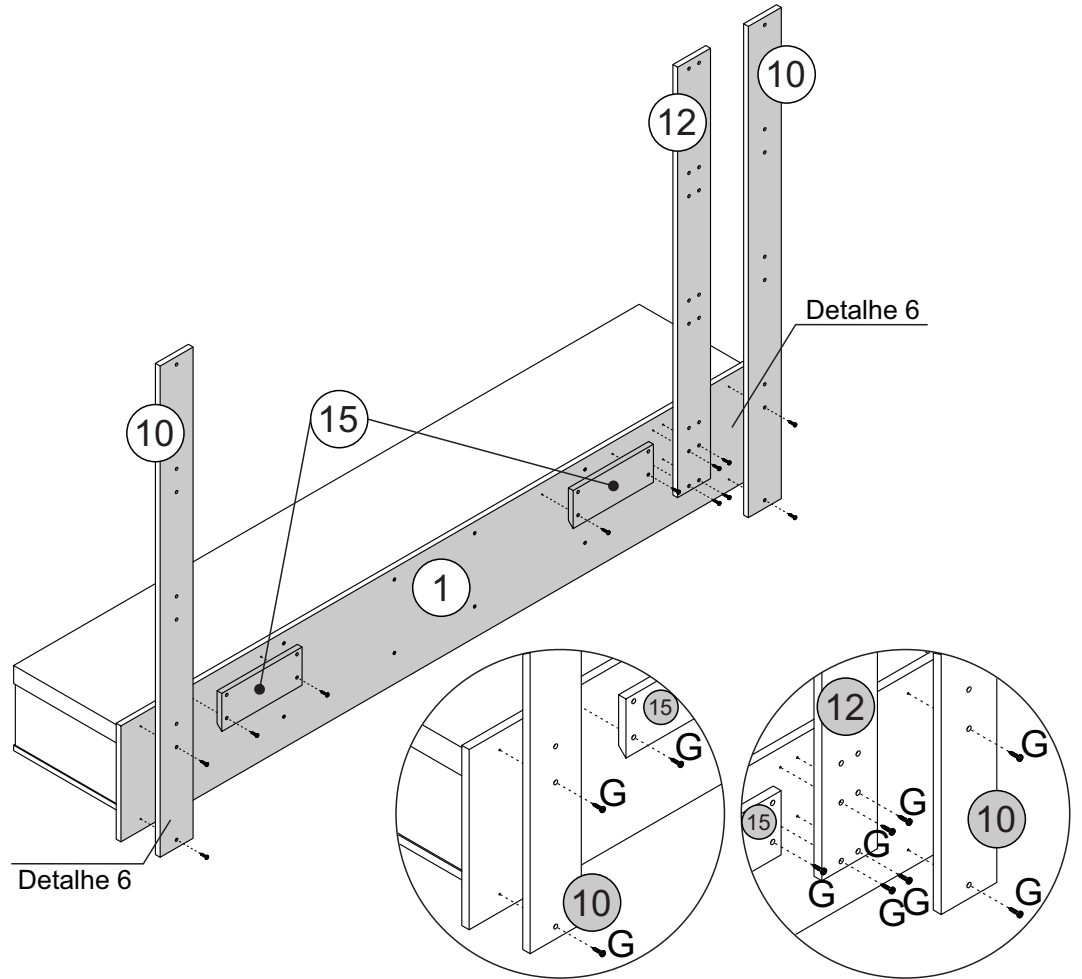
Detalhe 6 Detalle/Detail
