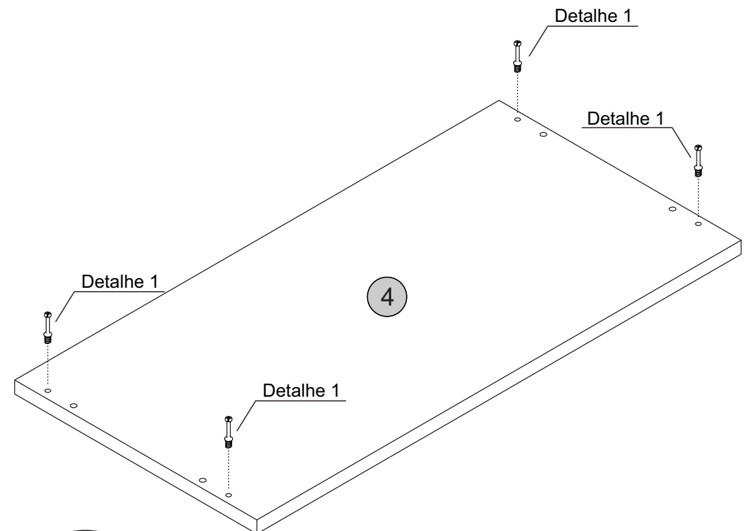
Detalhe 1 Detalle/Detail
