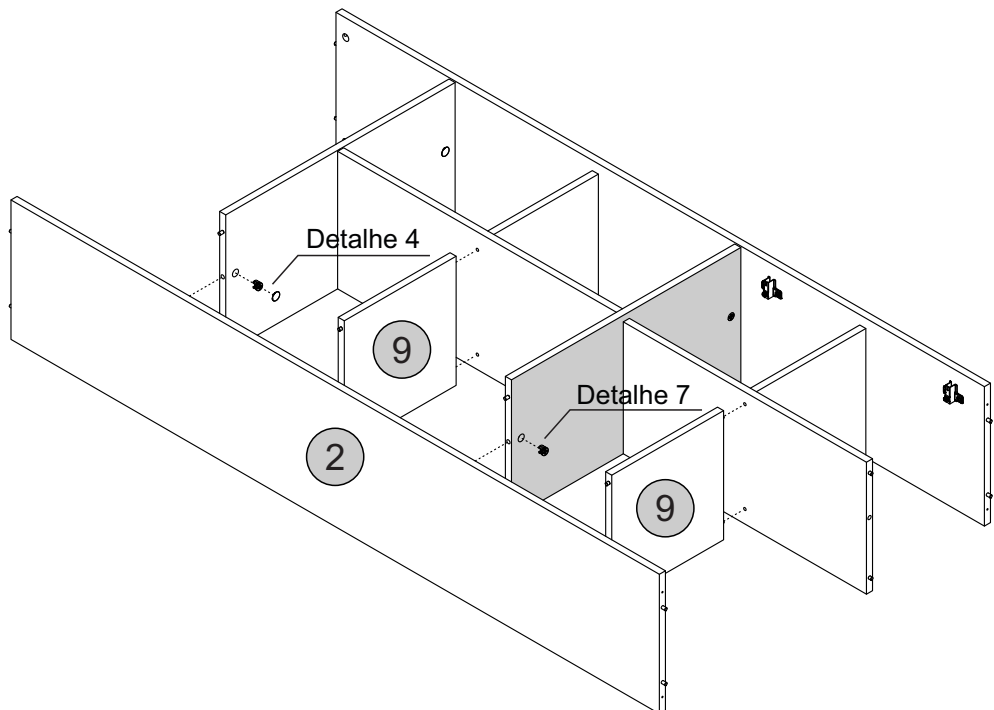
Detalhe 4 Detalle/Detail
